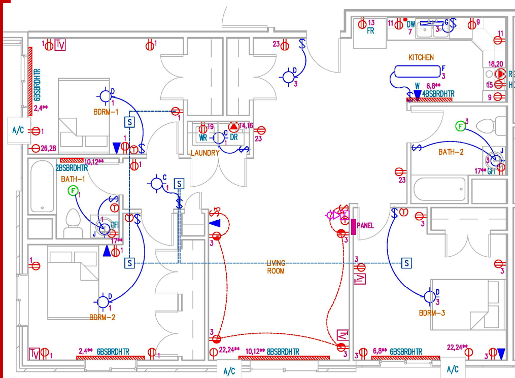
Typical 3-Bedroom Unit
